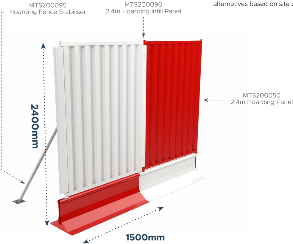
2m and 2.4m Hoarding panels
